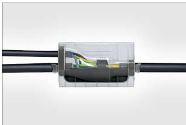
Parallel branch joint PAH-4 PUR771.
