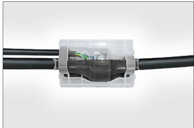
Parallel branch joint PAH-2 PUR771.
